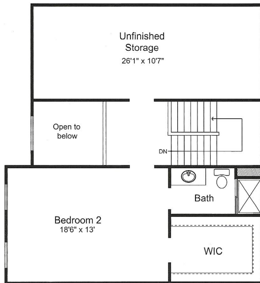
SECOND FLOOR STANDARD
