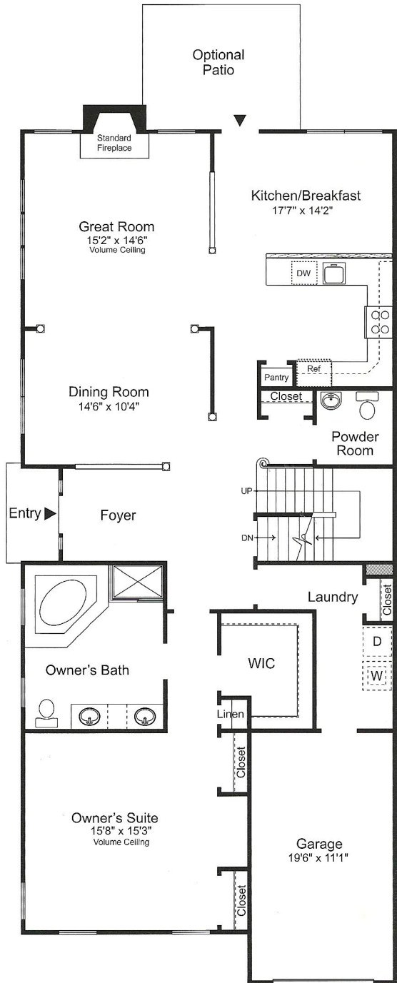
FIRST FLOOR STANDARD
